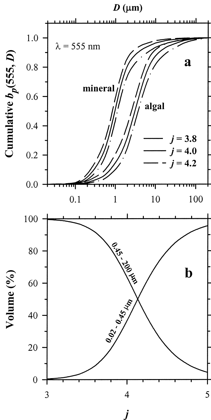
Fig. 4. (a) Theoretical relationship between the cumulative b_p(D) at \lambda = 555 nm and particle diameter ( D ) for typical mineral and algal particles and for different slopes of the size distribution (see text for details). (b) Calculated volume of particles with diameter between 0.02 and 0.45 \mu\text{m} and between 0.45 and 200 \mu\text{m} , relative to the sum of these two fractions, plotted as a function of the slope of a Junge-type particle size distribution ( j ).
