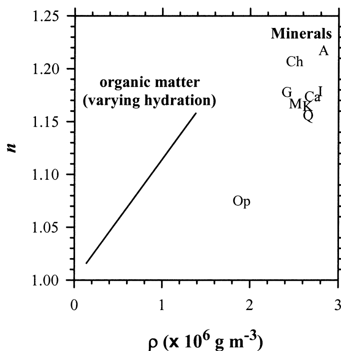
Fig. 7. The index of refraction relative to seawater for various minerals as a function of particle density. The n and \rho values (also listed in Table 6) are from Lide (2001). The n values are the arithmetic average of the values given for the two or three structure coordinate axes. The plotted minerals are aragonite (A), calcite (Ca), chlorite (Ch), gibbsite (G), illite (I), kaolinite (K), montmorillonite (M), opal (Op), and quartz (Q). The theoretical relationship between n and \rho is also shown for organic matter (see text for details).
