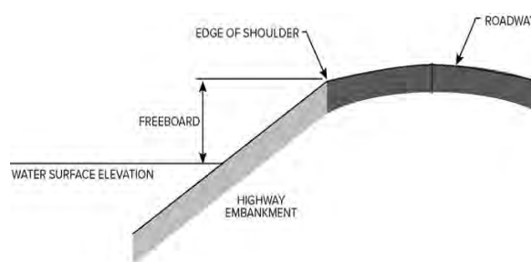
Figure 7. Illustration of roadway freeboard.
